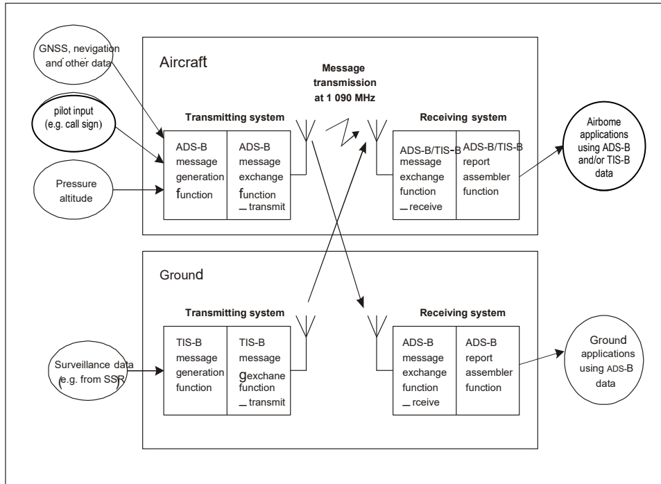
Figure 5-1. ADS-B/TIS-B system functional model
