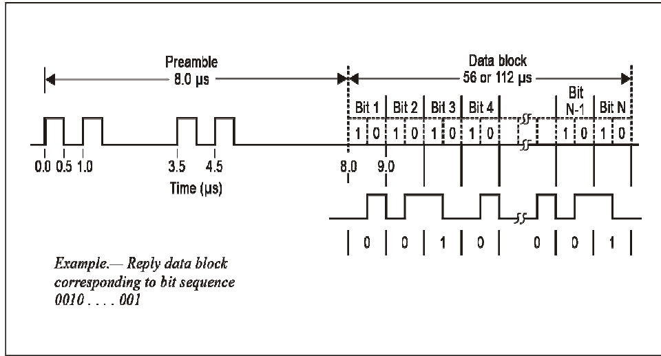
Figure 3-6. Mode S reply
