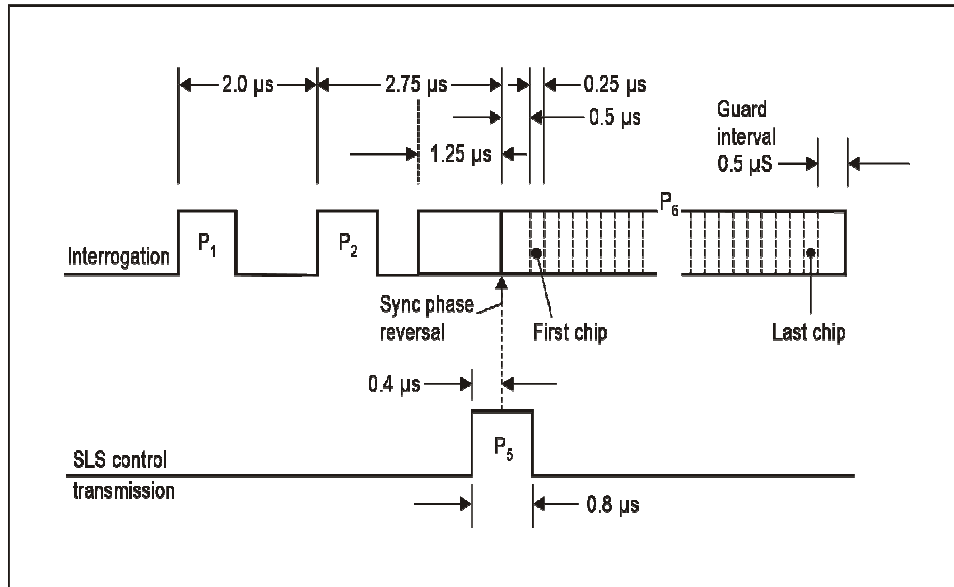
Figure 3-4. Mode S interrogation pulse sequence
