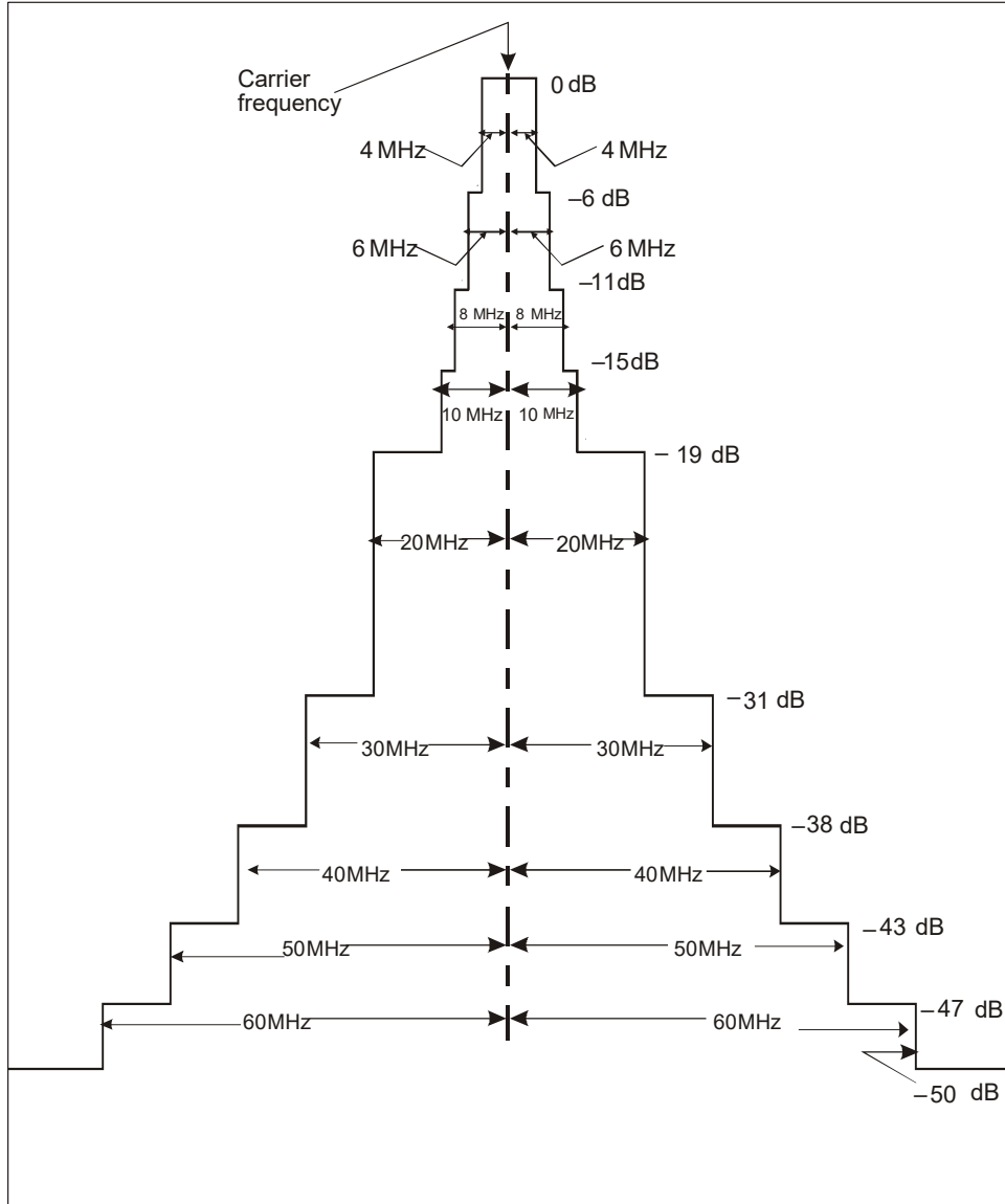
Figure 3-2. Required spectrum limits for interrogator transmitter
