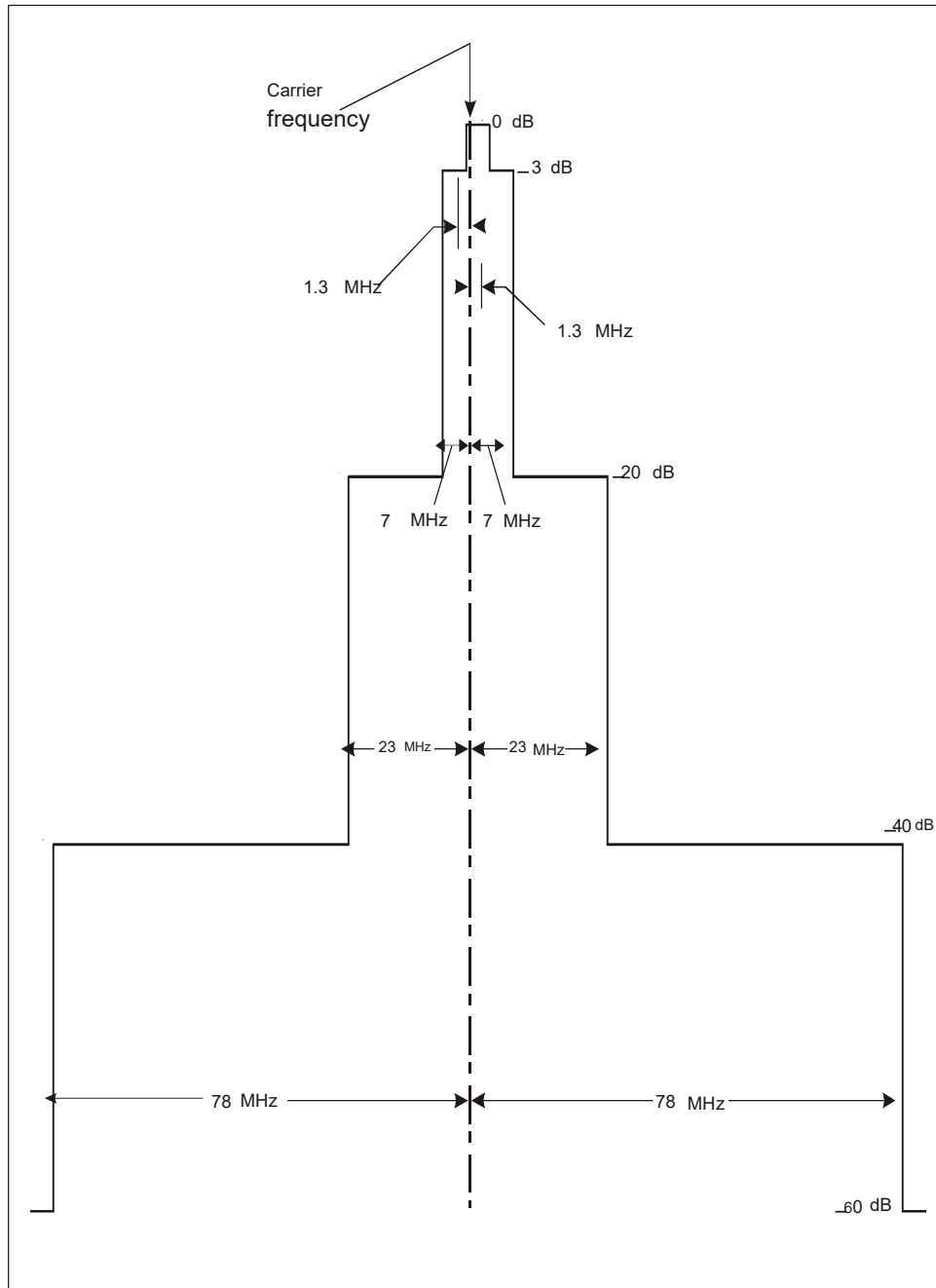
Figure 3-5. Required spectrum limits for transponder transmitter
