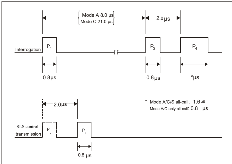
Figure 3-3. Intermode interrogation pulse sequence
