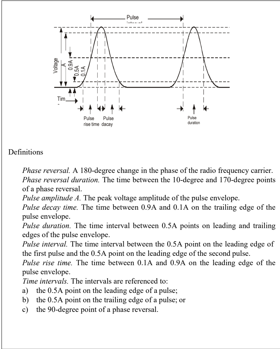
Figure 3-1. Definitions of secondary surveillance radar waveform shapes, intervals and the reference point for sensitivity and power.
