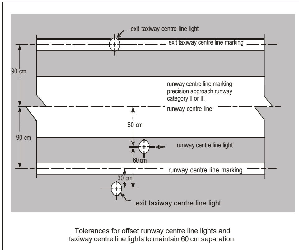
Figure 5-27. Offset runway and taxiway centre line lights
