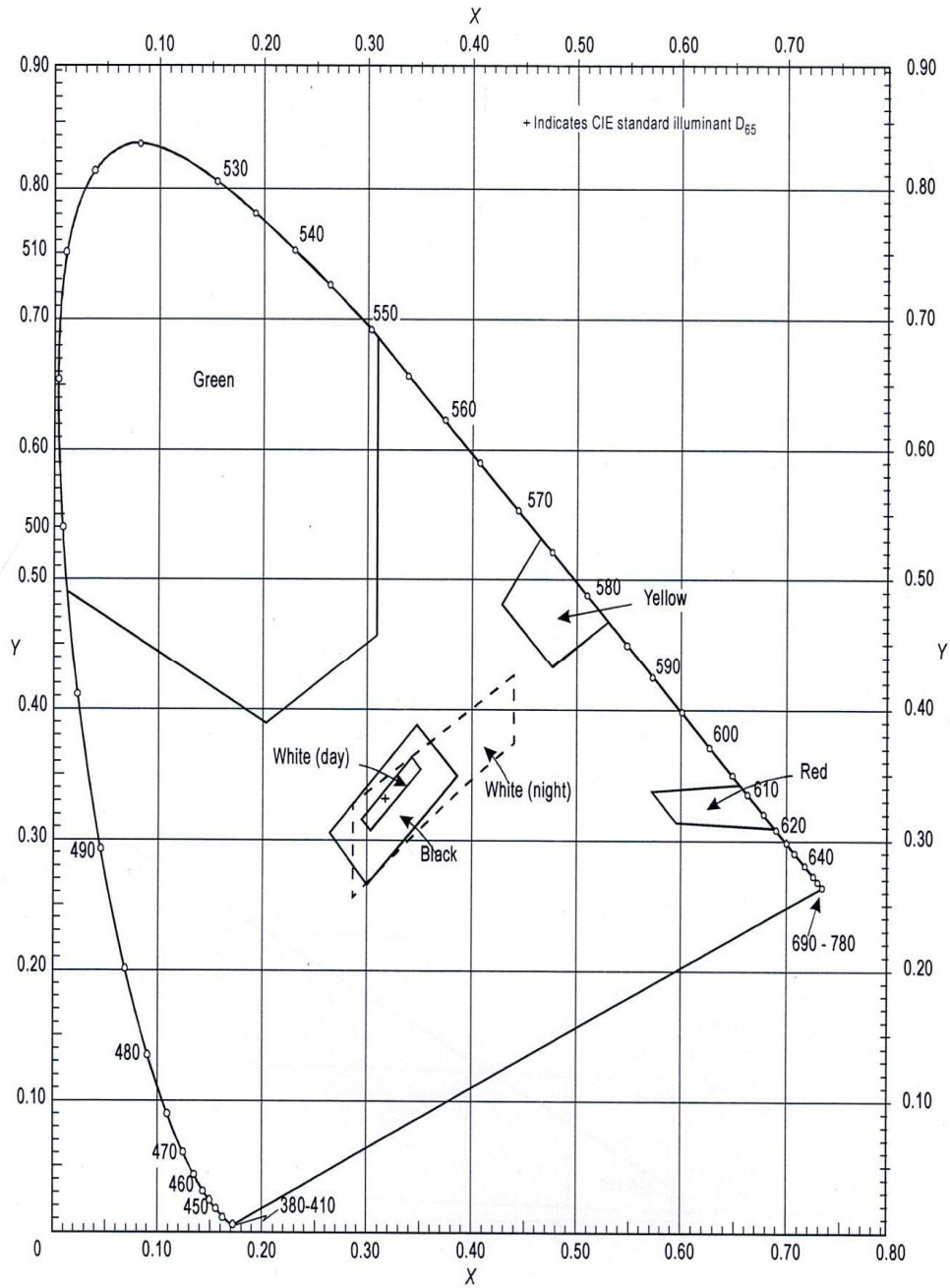
Figure A1-4. Colours of luminescent or transilluminated (internally illuminated) signs and panels
