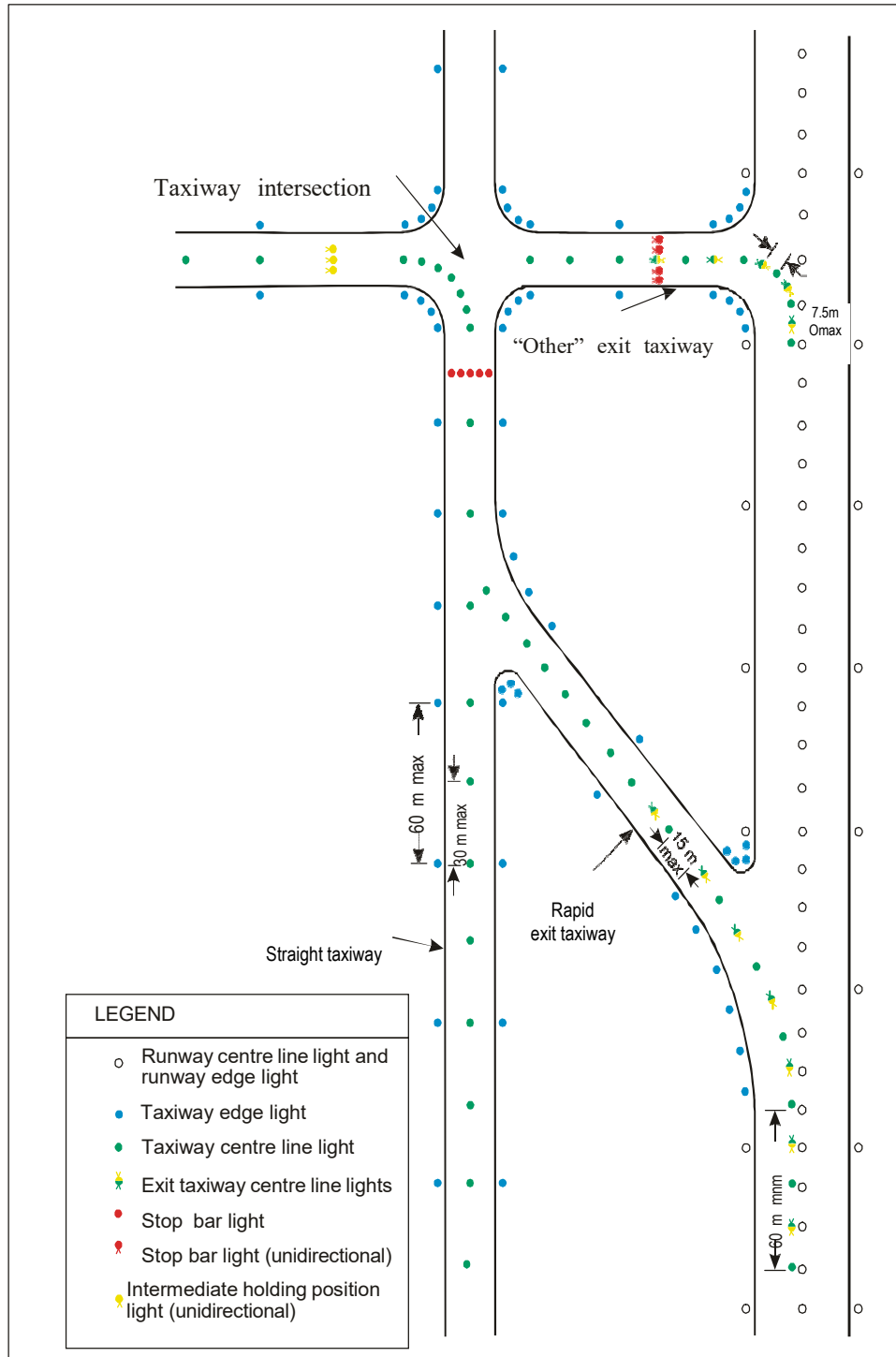
Figure 5-26. Taxiway lighting
