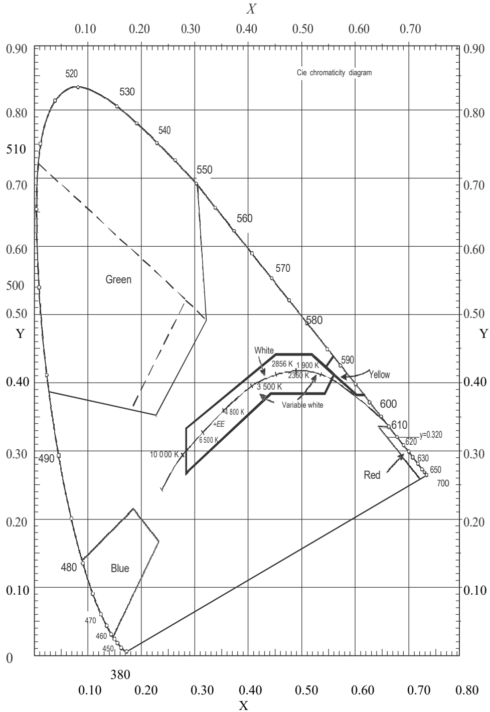
Figure A1-1a. Colours for aeronautical ground lights (filament-type lamps)
