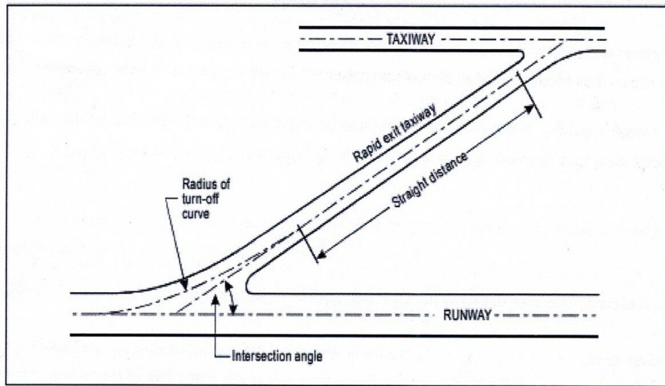
Figure 3-2. Rapid exit taxiway
