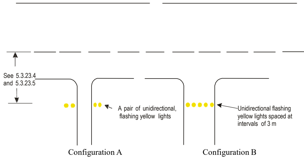
Figure 5-29. Runway guard lights
