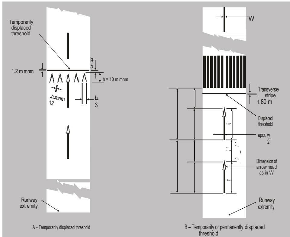
Figure 5-4. Displaced threshold markings
