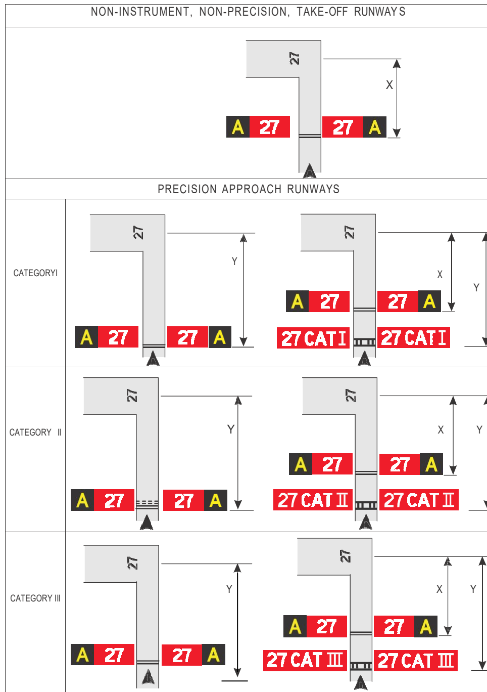
Figure 5-32. Examples of sign positions at taxiway/runway intersections
