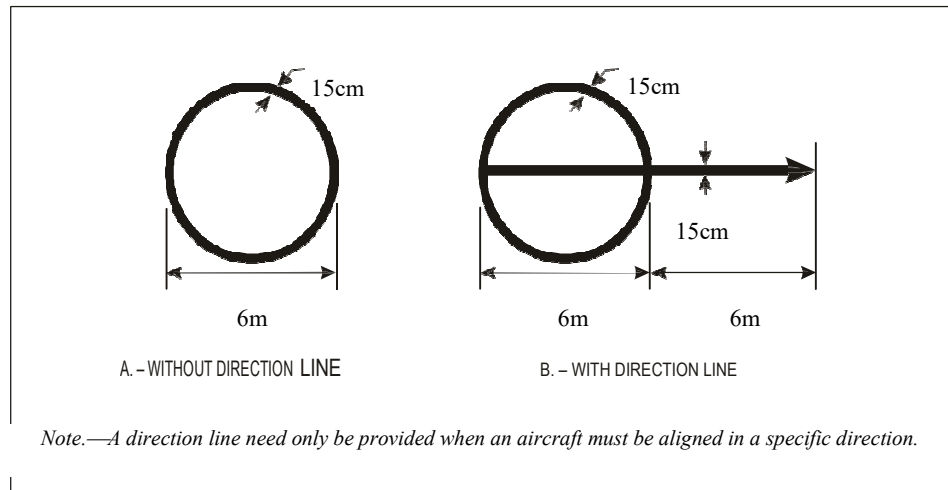
Figure 5-9. VOR aerodrome checkpoint marking
