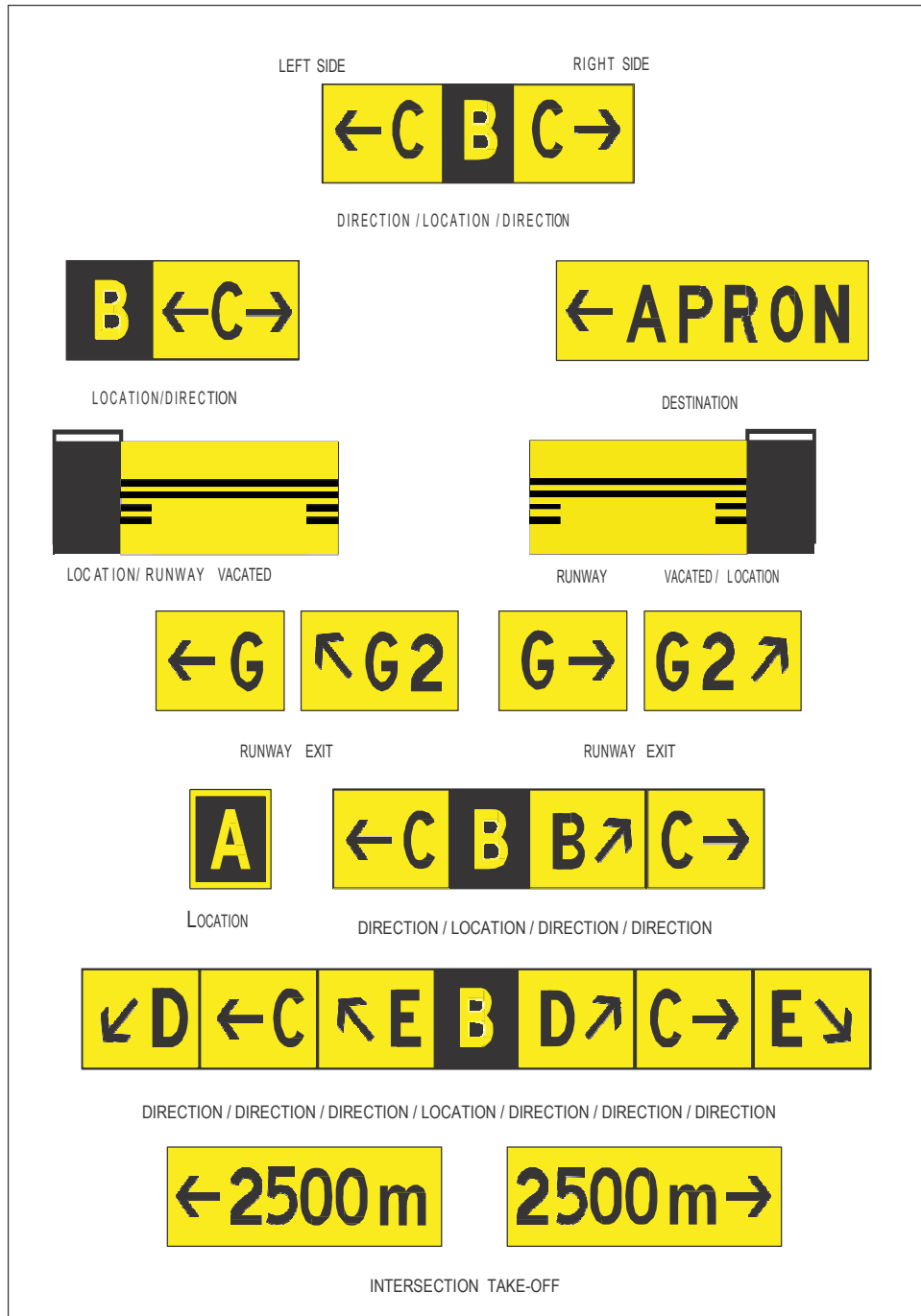
Figure 5-31. Information signs
