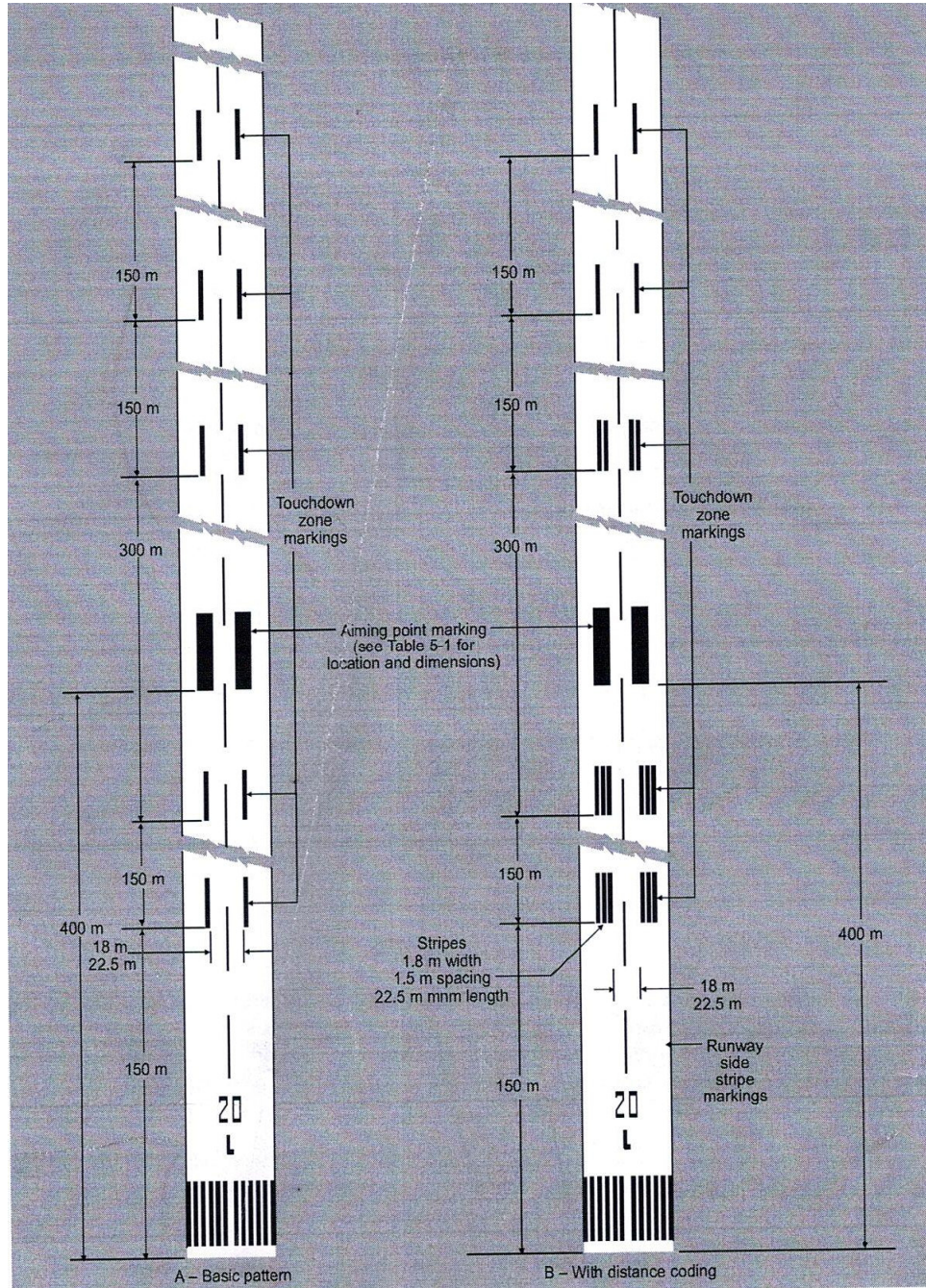
Figure 5-5. Aiming point and touchdown zone markings (illustrated for a runway with a length of 2400 m or more)
