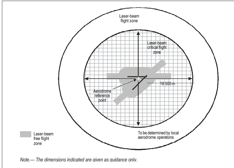
Figure 5-11. Protected flight zones
