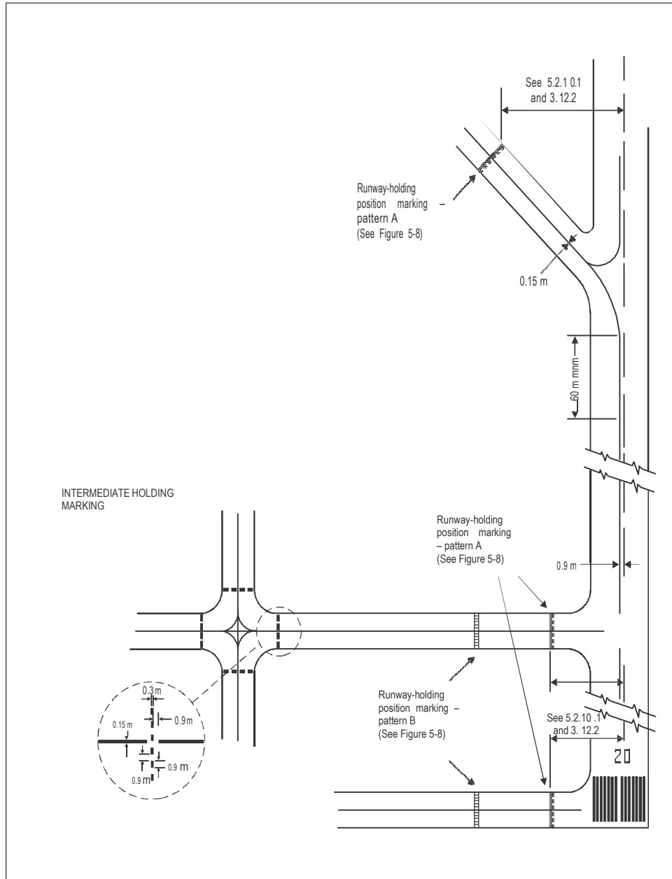
Figure 5-6. Taxiway markings (shown with basic runway markings)
