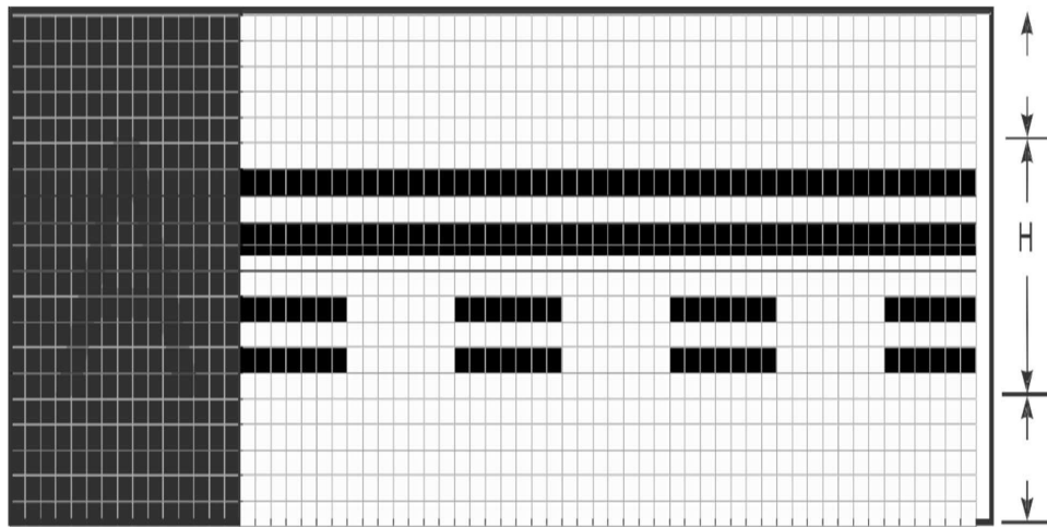
Runway vacated sign (with typical location sign)
