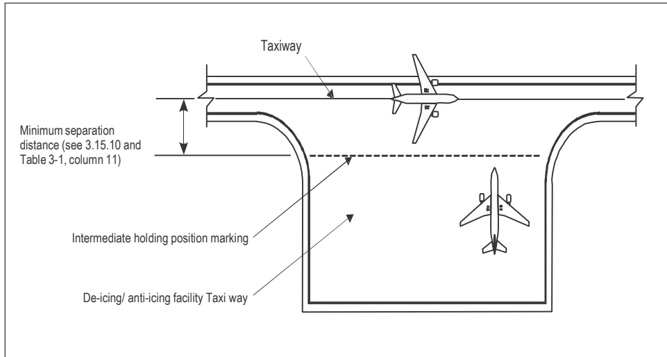
Figure 3-4. Minimum separation distance on a de-icing/anti-icing facility
