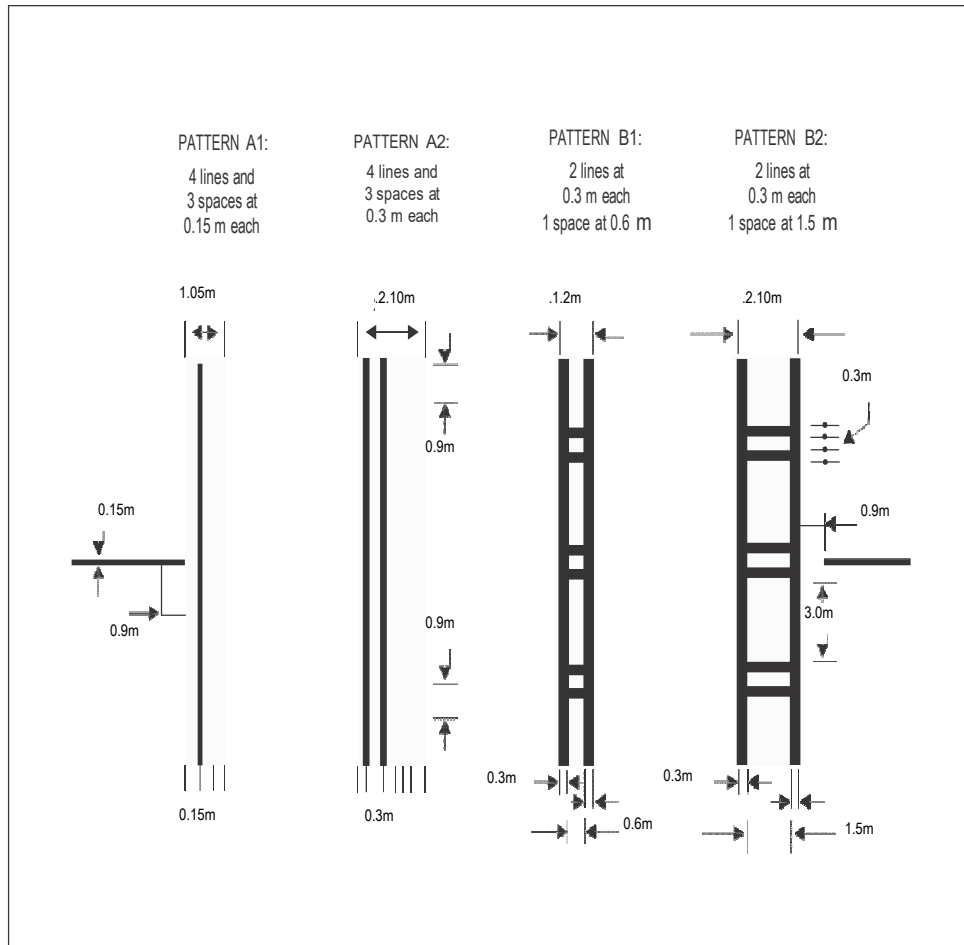
Figure 5-8. Runway-holding position markings
