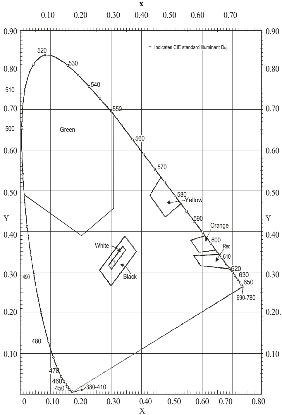
Figure A1-2. Ordinary colours for markings and externally illuminated signs and panels
