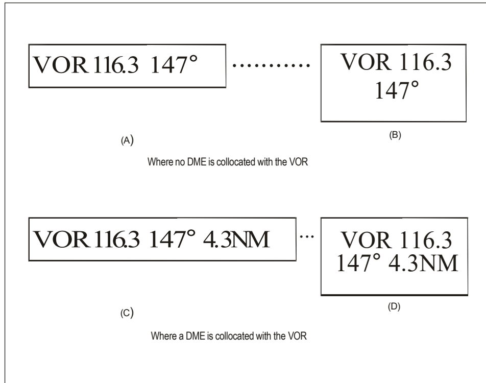
Figure 5-33. VOR aerodrome checkpoint sign
