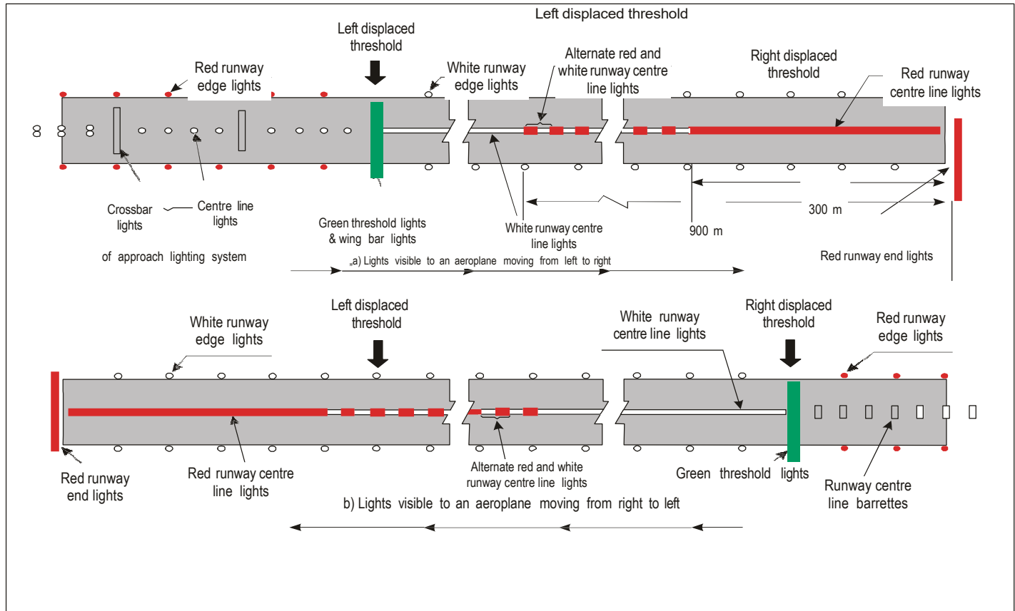
Example shows lighting on a runway having displaced thresholds at each end and a precision approach category I lighting system serving the left displaced threshold
