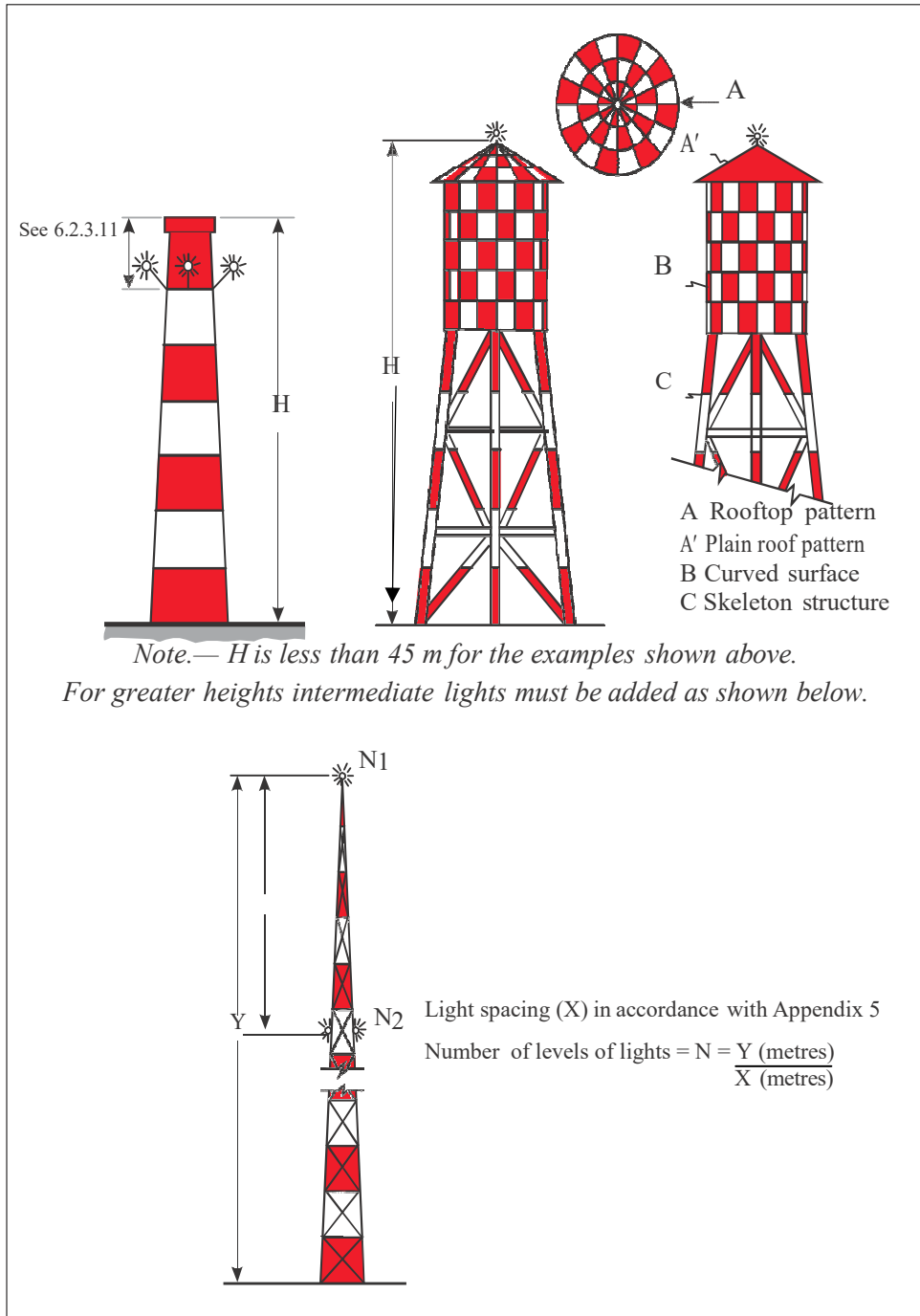
Figure 6-2. Examples of marking and lighting of tall structures
