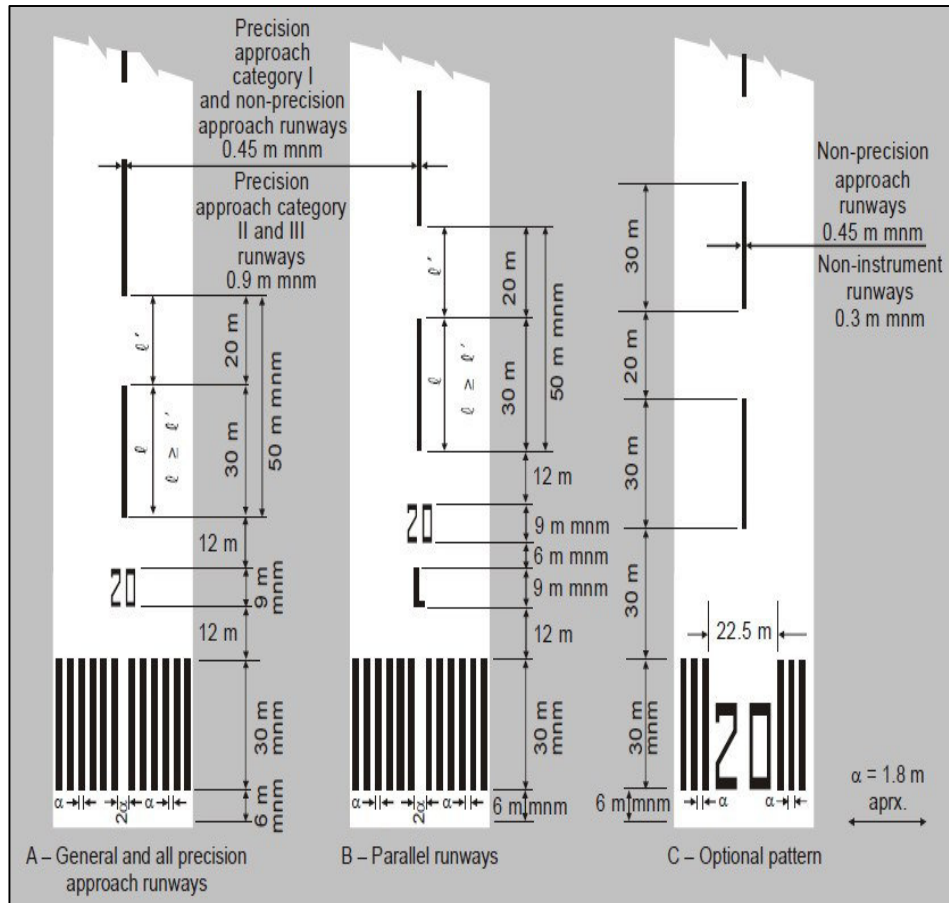
Figure 5-2. Runway designation, centre line and threshold markings
