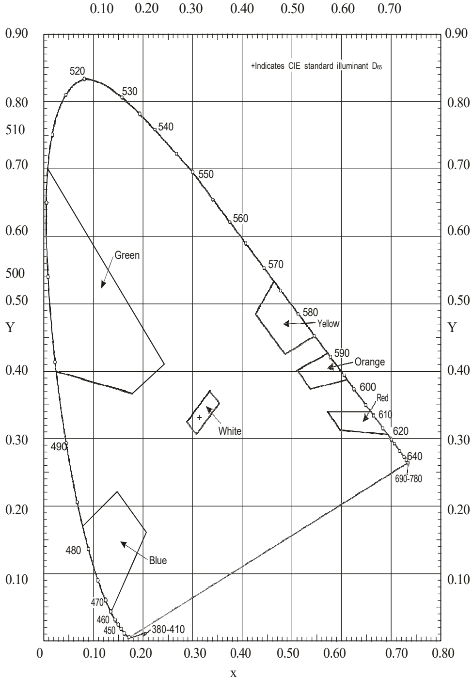
Figure A1-3. Colours of retroreflective materials for markings, signs and panels
