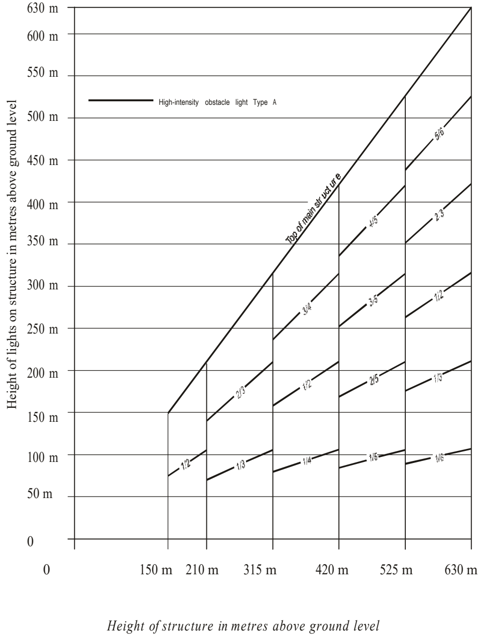
Figure A5-6. High-intensity flashing-white obstacle lighting system, Type A
