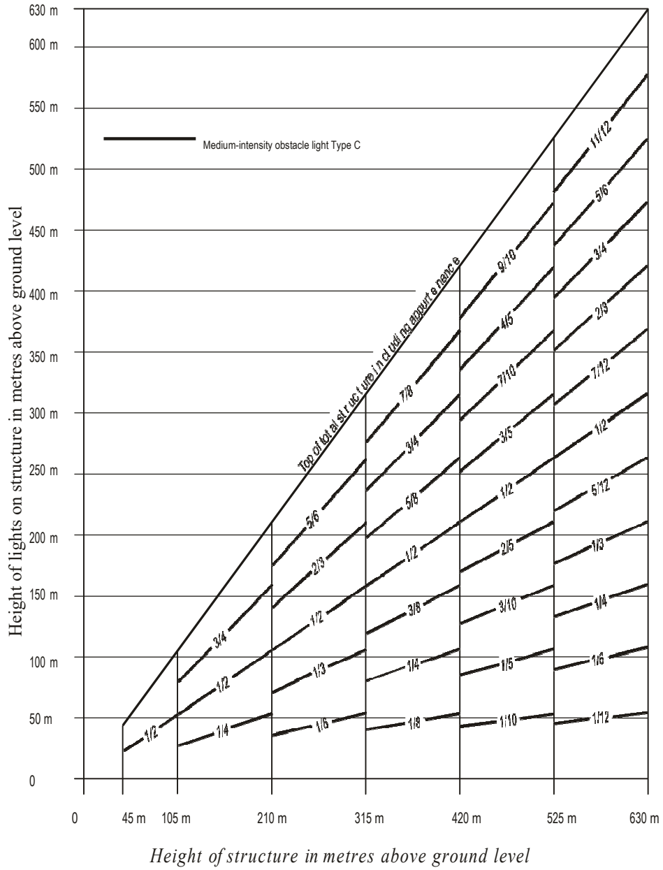
Figure A5-3. Medium-intensity fixed-red obstacle lighting system, Type C
