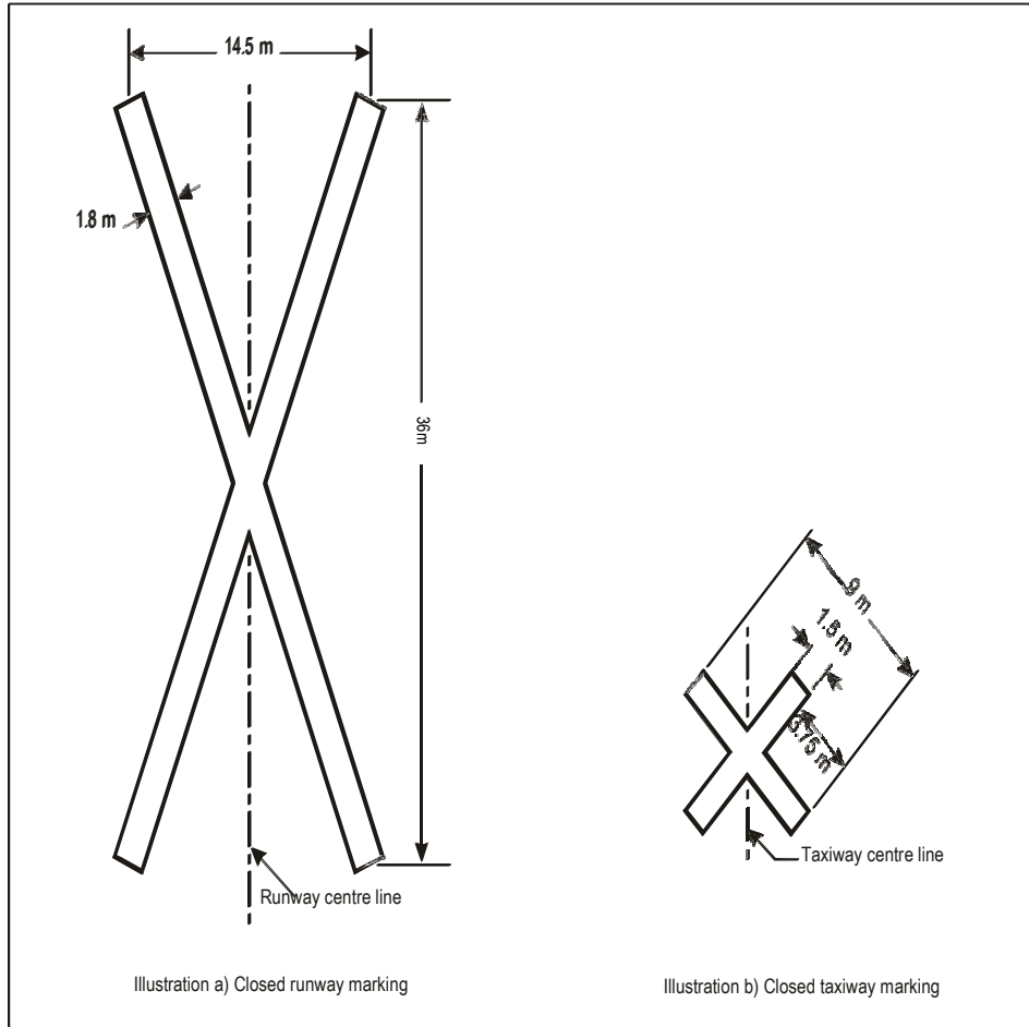
Figure 7-1. Closed runway and taxiway markings
