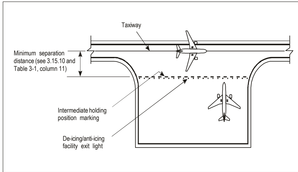
Figure 5-28. Typical remote de-icing/anti-icing facility
