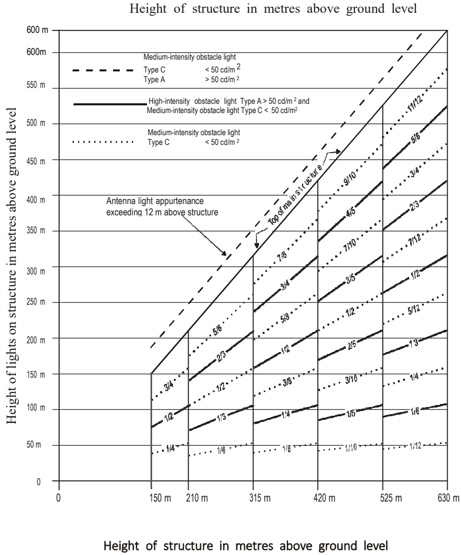
Figure A5-8. High-/medium-intensity dual obstacle lighting system, Type A/Type C
