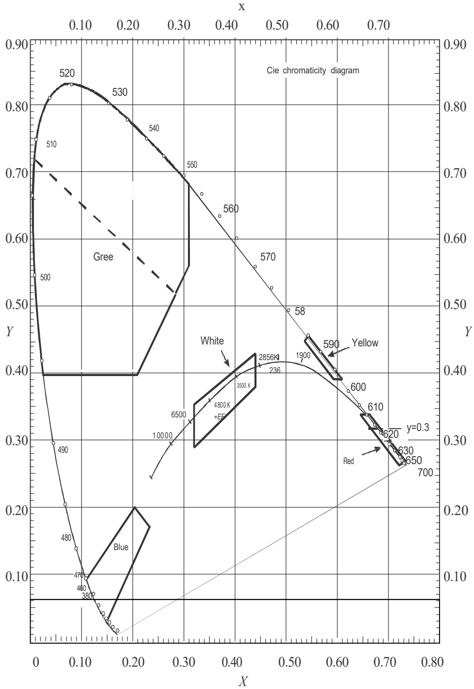
Figure A1-1b. Colours for aeronautical ground lights (solid state lighting)
