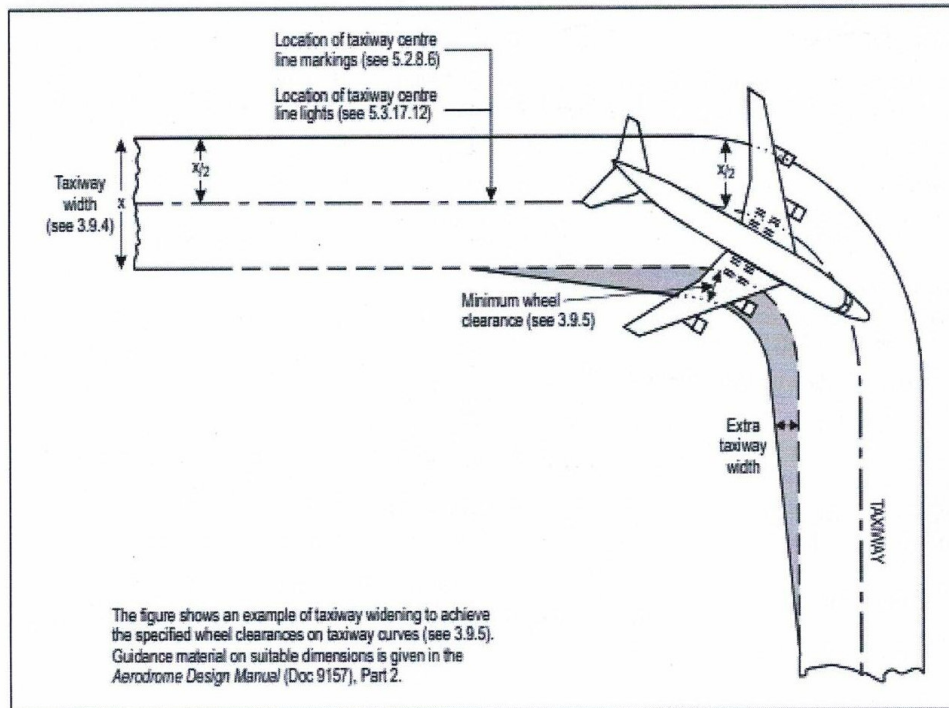
Figure 3-2. Taxiway curve
