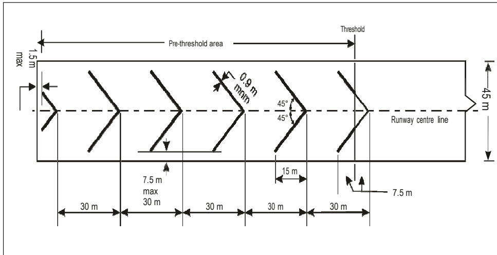
Figure 7-2. Pre-threshold marking
