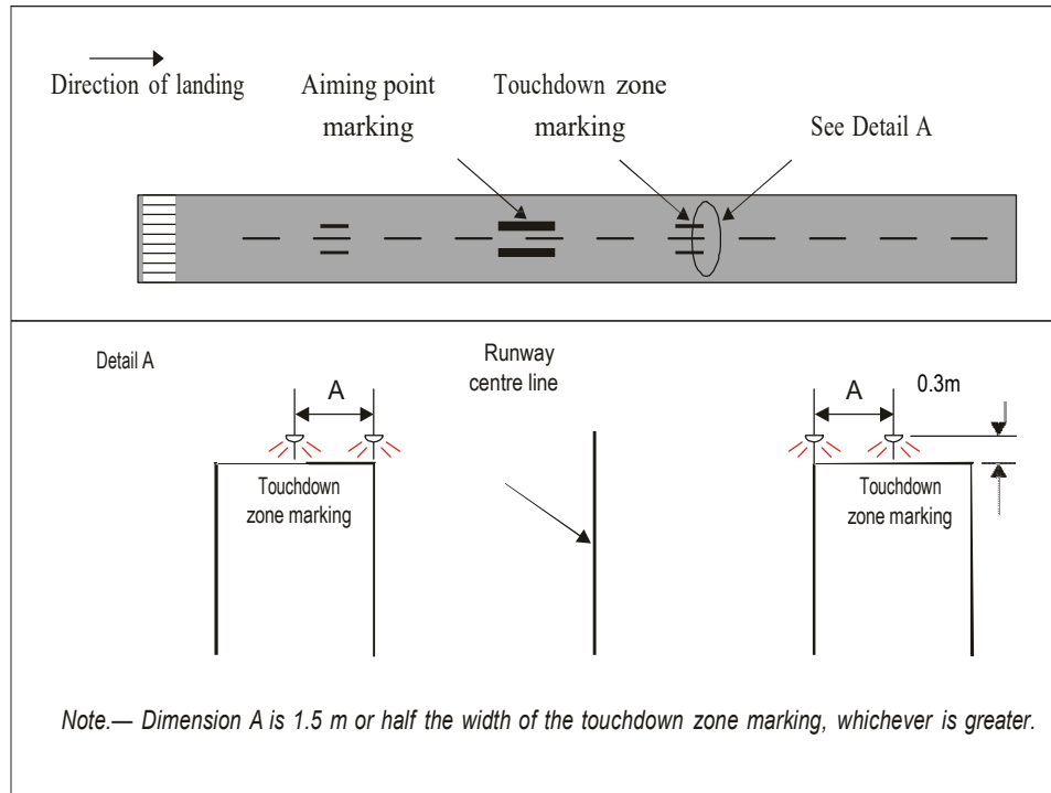
Figure 5-24. Simple touchdown zone lighting
