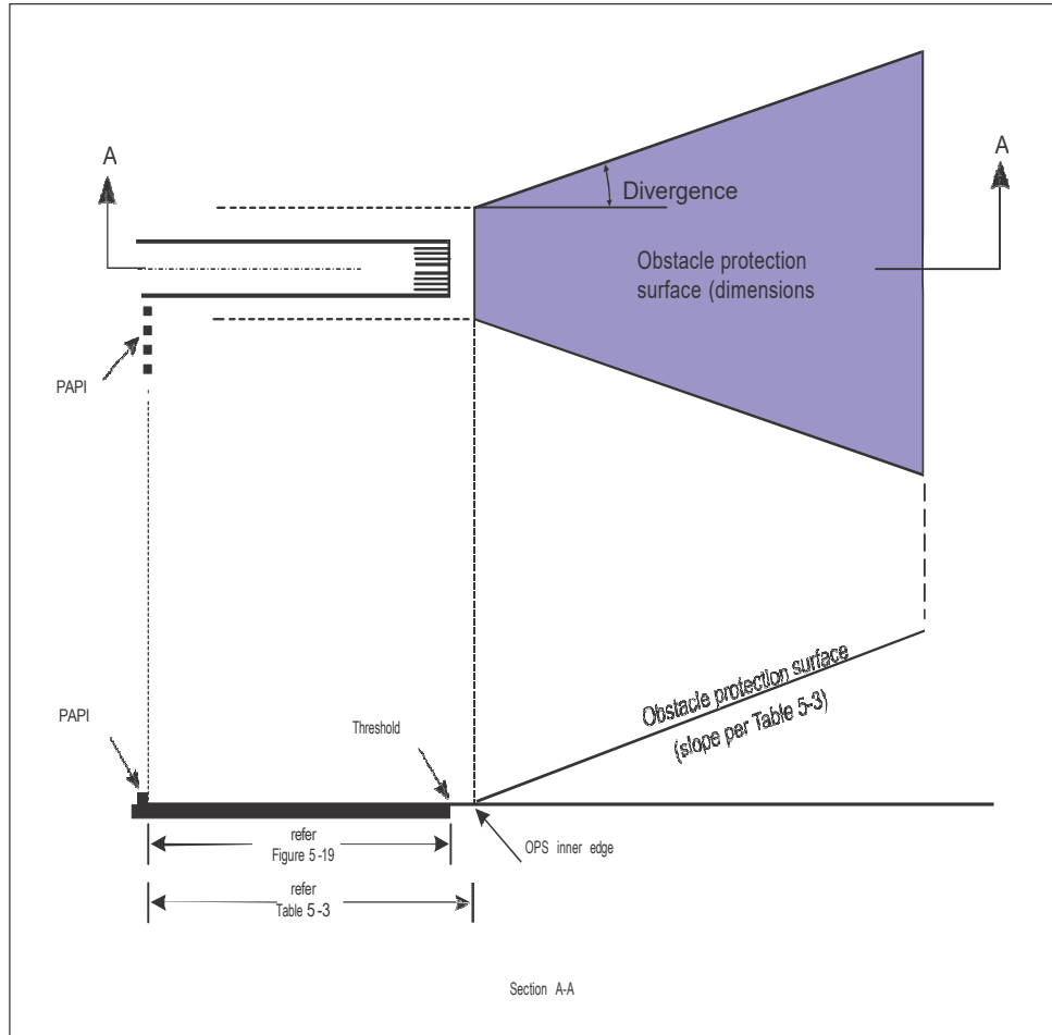
Figure 5-21. Obstacle protection surface for visual approach slope indicator systems
