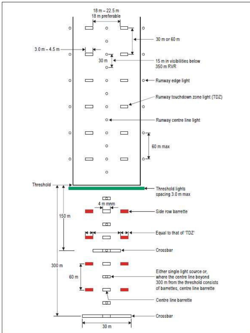
Figure 5-15. Inner 300 m approach and runway lighting for precision approach runways, categories II and III, where the serviceability levels of the lights specified as maintenance objectives in Chapter 10 can be demonstrated
