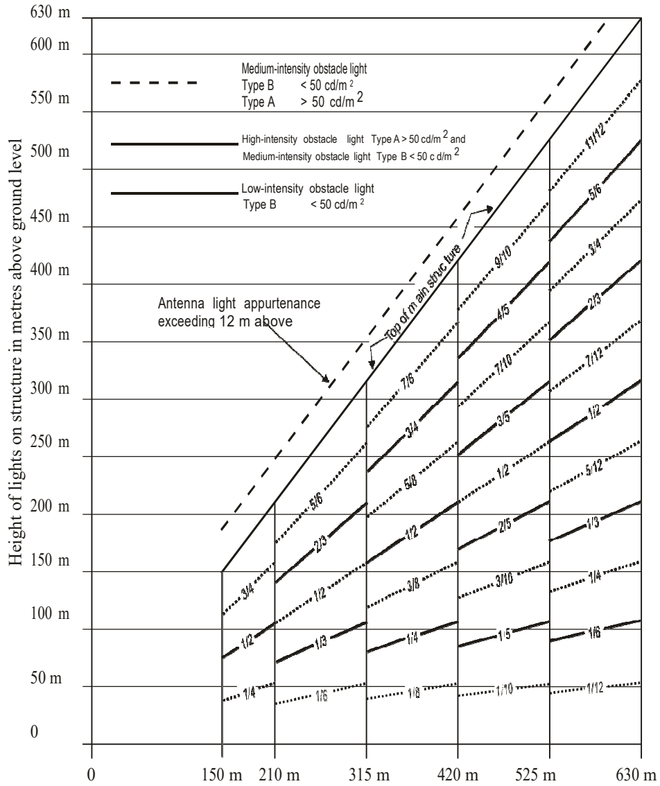
Figure A5-7. High-/medium-intensity dual obstacle lighting system, Type A/TypeB
