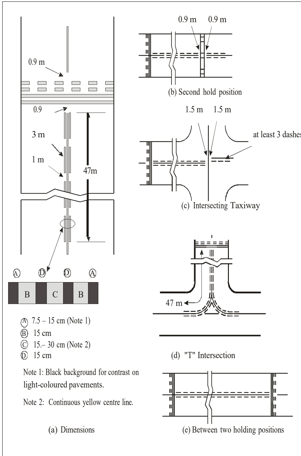
Figure 5-7. Enhanced taxiway centre line marking
