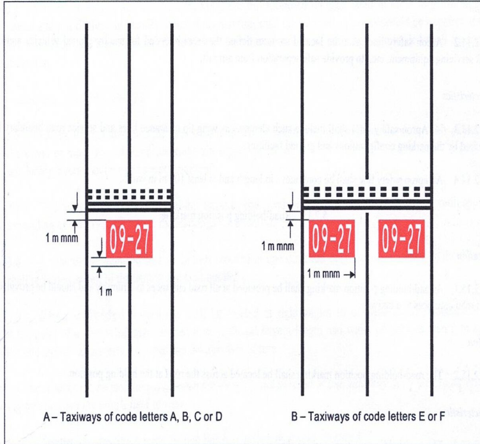
Figure 5-10. Mandatory instruction marking
