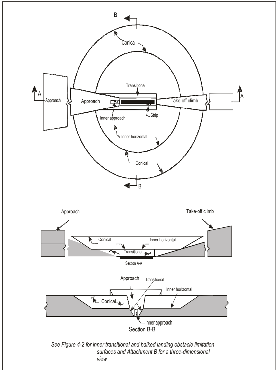
Figure 4-1. Obstacle limitation surfaces
