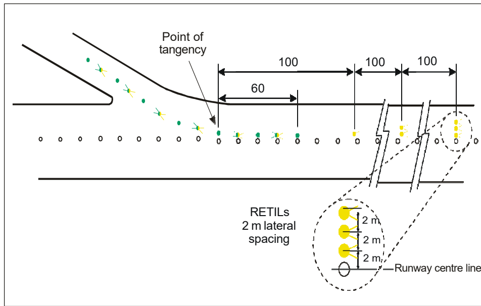
Figure 5-25. Rapid exit taxiway indicator lights (RETILS)
