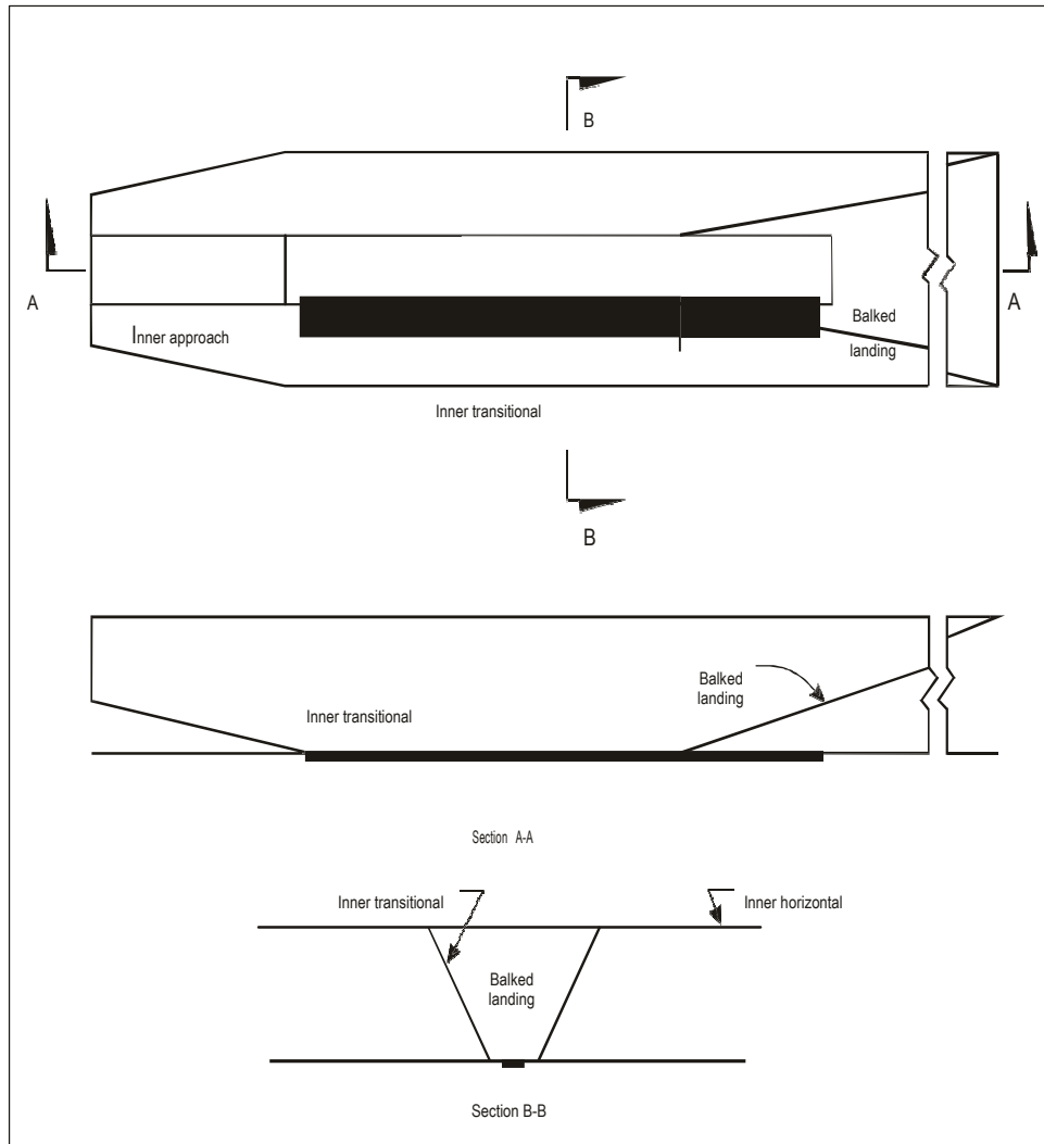
Figure 4-2. Inner approach, inner transitional and balked landing obstacle limitation surfaces
