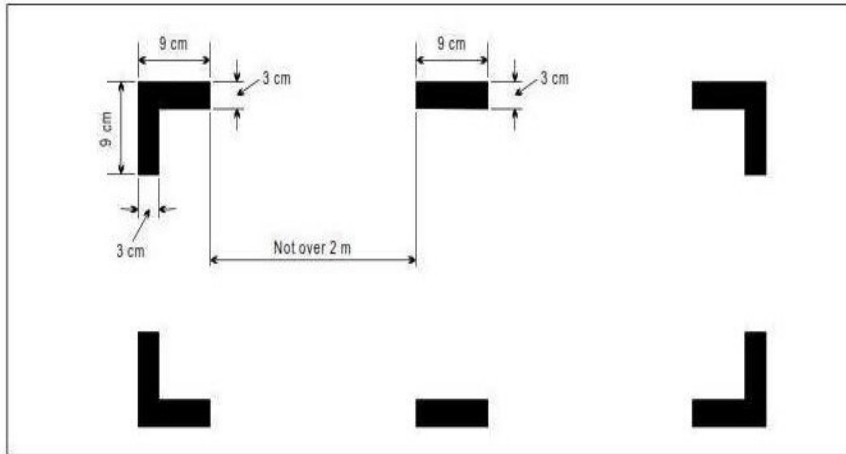
MARKING OF BREAK-IN POINTS (see-6.2.4)
